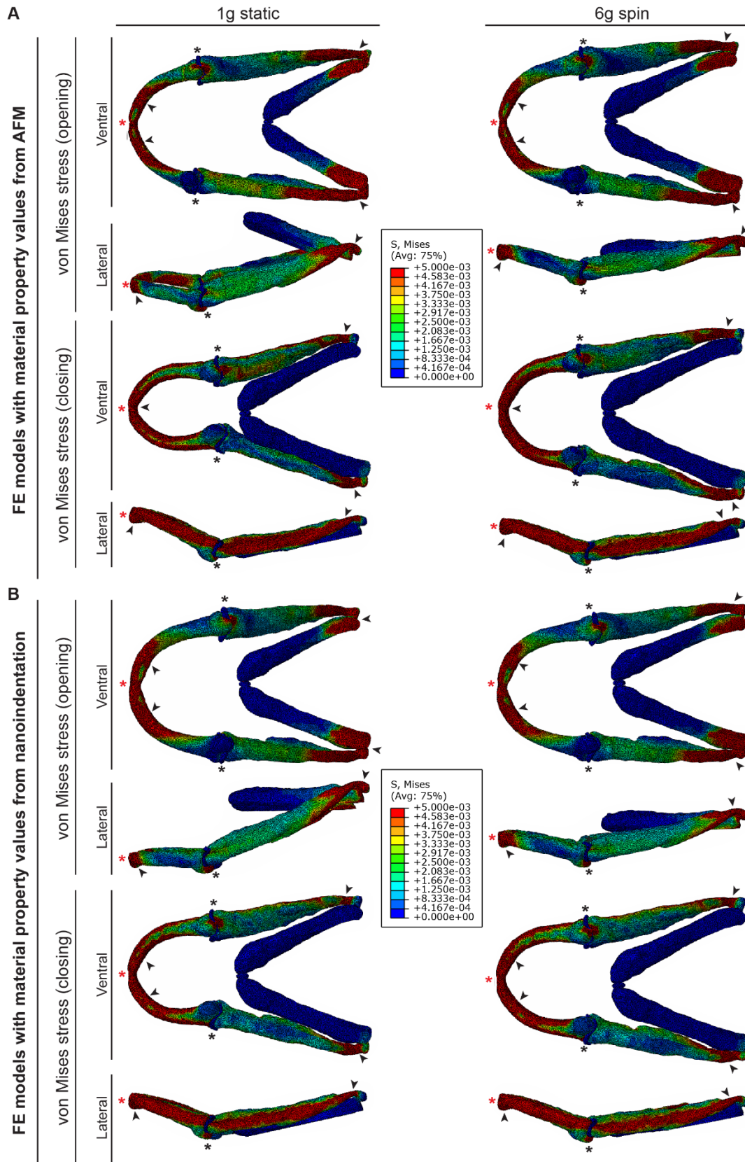
Fig. c. Altered extracellular matrix (ECM) characteristics could result from altered stress distribution in the lower jaw following hypergravity exposure. a) Finite element (FE) models of von Mises stress
