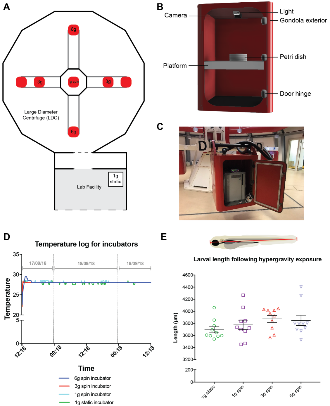
Fig. a. Setup of experiment in large diameter centrifuge (LDC). a) Floorplan of Life, Physical Sciences and Life Support Laboratory, including the LDC and lab area used for the project. Red boxes = gondola, white boxes = experiment areas external to LDC. b) Computer aided design (CAD) drawing of setup within a gondola (incubator not shown). c) Image of gondola setup with incubator. d) Graph showing temperature fluctuations during the course of the experiment. e) Quantification of larval length following 48 hours in hypergravity ( n = 10 for all). Location of measurements taken is marked on schematics above each graph. Data are means with standard errors of the mean (SEM).
