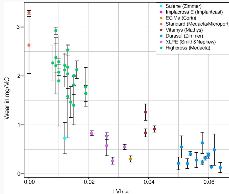
Fig. 5 Wear in dependence of TVI_{1370} , as determined in a modified pin-on-disk test. Dots mark mean values of n = 3 samples per liner/cup, colour-coded by brand. The error margin corresponds to the SD. There is a correlation between TVI and in vitro wear, with overall lower wear for higher TVI. TVI, trans-vinylene index; XLPE, cross-linked polyethylene.
