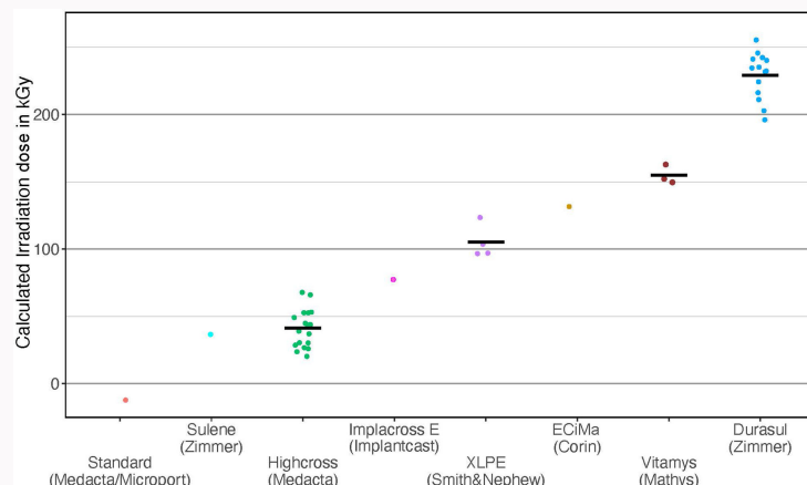
Fig. 2 The TVI_{1370} value measured on all the samples was converted to the absorbed irradiation dose, using the calibration curve for remelted highly cross-linked polyethylene (HXLPE) published previously. Results are grouped by product, with individual points indicating individual values. The horizontal bar indicates the mean. TVI, trans-vinylene index.
