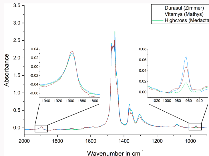
Fig. 6 Exemplary Fourier-transform infrared (FTIR) spectra of the cross-linked polyethylene (XLPE) Highcross, Durasul, and Vitamys, the latter being vitamin E blended. The trans-vinylene index (TVI) is the ratio between the area under the peak at 965\text{ cm}^{-1} , considered characteristic for vinylenes, and a normalization peak at 1370\text{ cm}^{-1} (acc. ASTM F2381-19) or 1900\text{ cm}^{-1} . Note the differences between the materials as well as the relevance of minor differences, with a potentially larger effect on the results.
